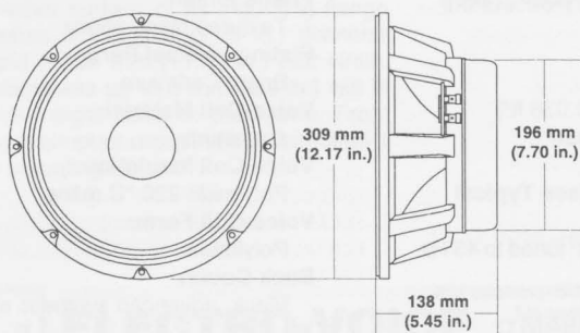
FIGURE 5 — DL12Sb Dimensions
