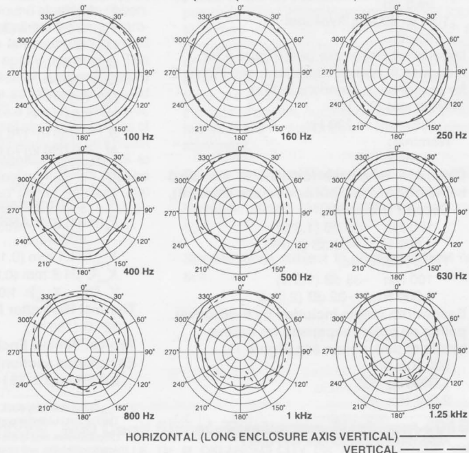
FIGURE 9 — DL12Sb Polar Response (TL12-1E enclosure)
