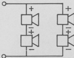
FIGURE 2 Electrical Connections
