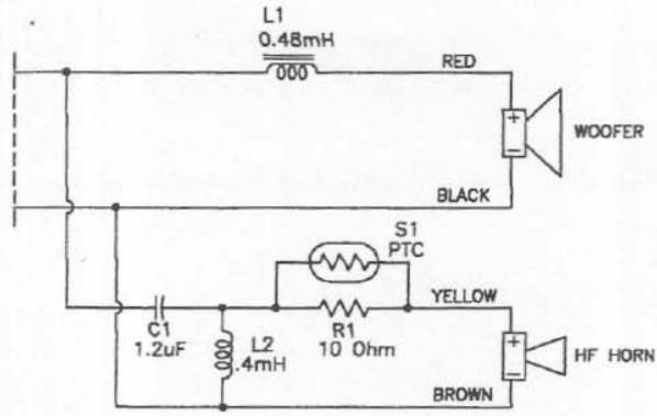
SCHEMATIC DIAGRAM
