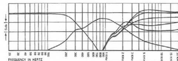
Crossover Response
