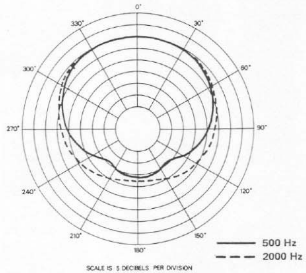
FIGURE 4 – Polar Response
