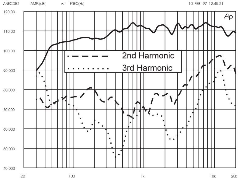
Figure 4—EVI-12 Distortion 10% power
