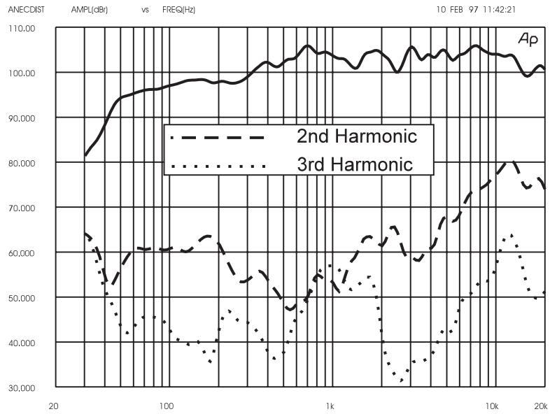
Figure 3—EVI-12 Distortion 1% power
