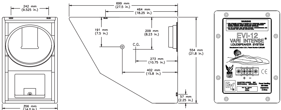
Figure 9—EVI-12 Dimensions
