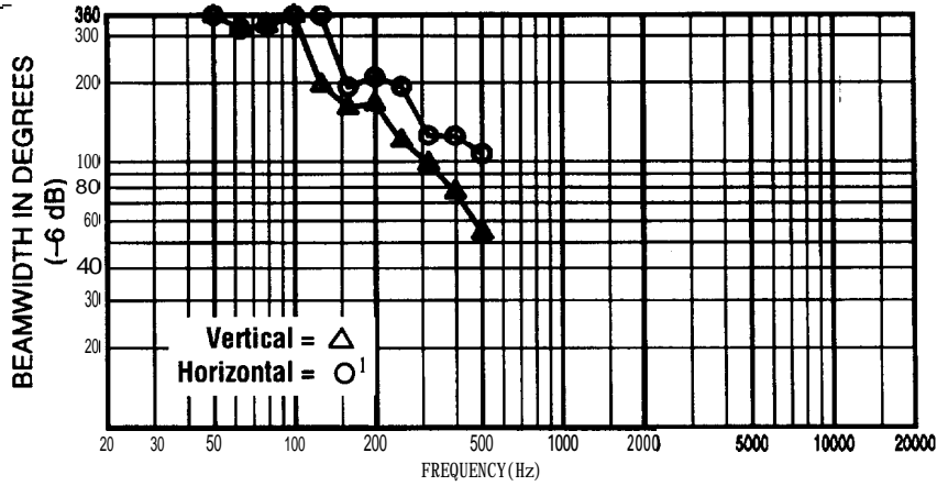
Figure 3-TL880P Beamwidth vs. Frequency
