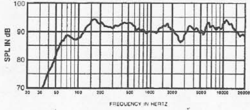
FIGURE 1 — T53 Axial Frequency Response, 1 Watt/1 Meter
